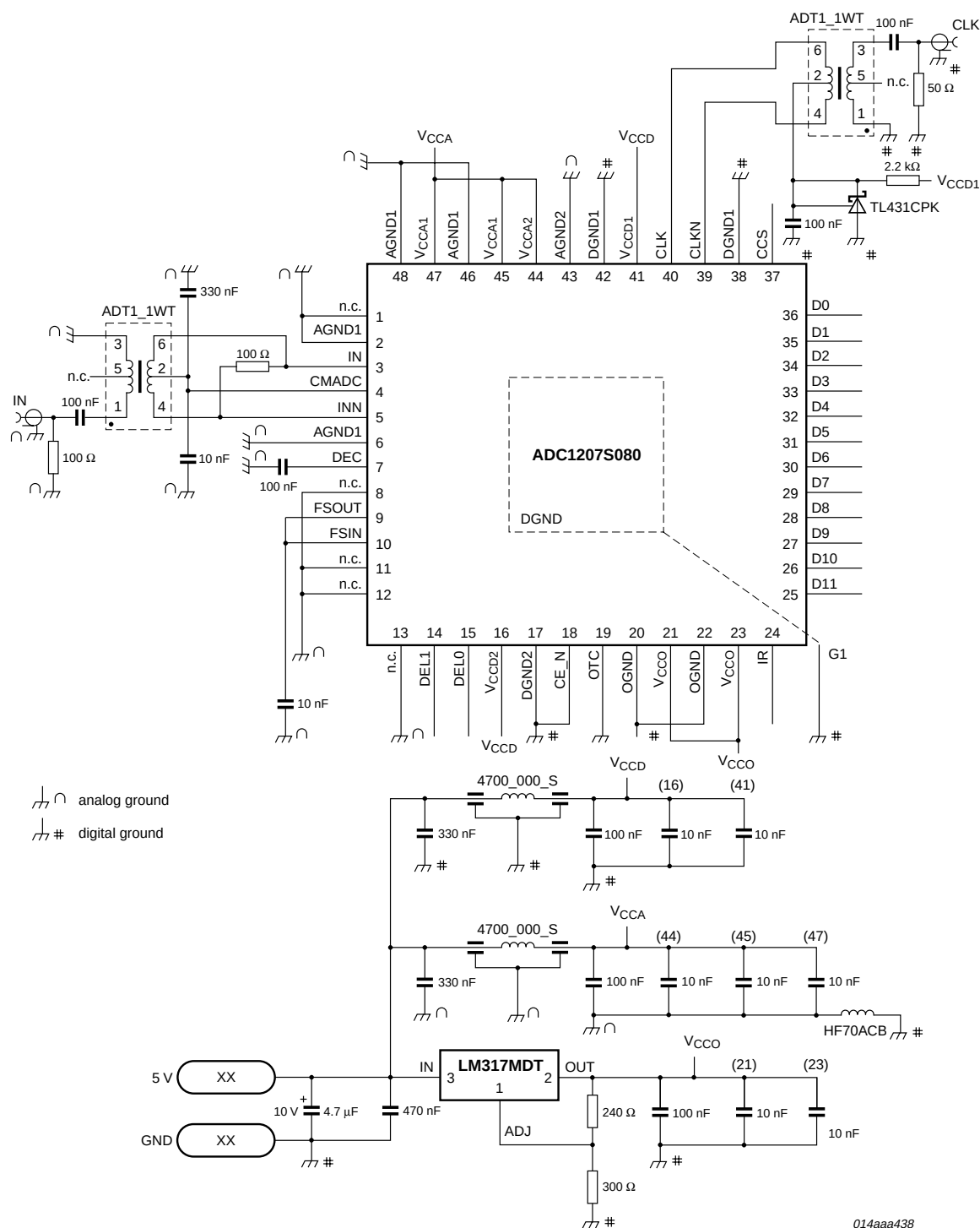
Fig 10. Application diagram
